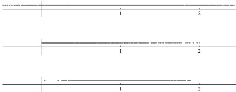
Figure 9: Three sets of randomly generated points
